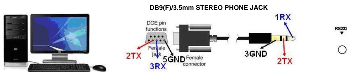
DB9(F)/3.5mm STEREO PHONE JACK
